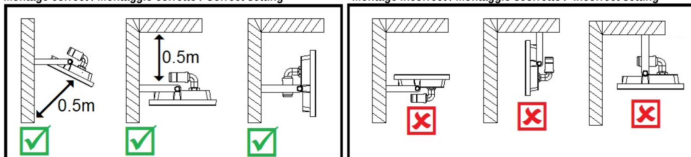
Fig.6- Installation recommandée / Montaggio raccomandato / Recommended installation
